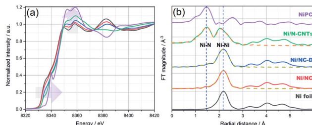
Fig. 3 (a) Normalized XANES spectra and (b) Fourier transform (FT) for k^2 -weighted EXAFS (solid lines) and the fit results (dashed lines) for Ni foil (black), Ni/NC (red), Ni/NC-D (blue), Ni/N-CNTs (green), and NiPc (purple), respectively. The blue vertical dashed lines at ca. 1.45 and 2.19 Å in (b) are to mark the position of Ni–N and Ni–Ni bonds, respectively. Details on the EXAFS analysis are provided in the ESI.†
