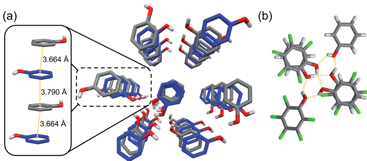
Fig. 1 View of (a) Ar–OH (blue)/ArF–OH (grey) co-crystal along the a -axis with the left inset illustrating \pi – \pi stacking distance of an Ar/ArF slip-stack along the b -axis, and (b) hydrogen-bonding hexameric unit.
