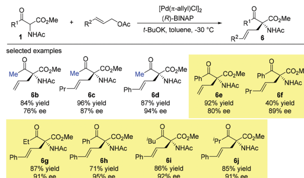
Scheme 31 Asymmetric allylation of α-acetamido-β-ketoesters.
