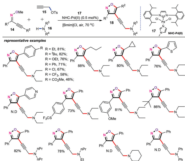
Scheme 7 Palladium-catalyzed three-component cascade cyclization/alkynylation.
