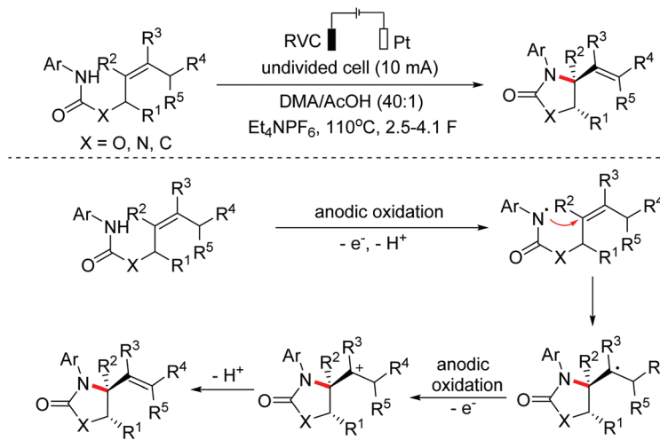
Scheme 60
