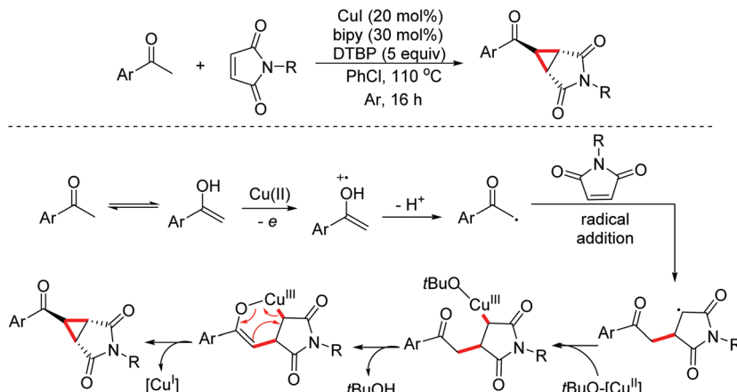
Scheme 49
