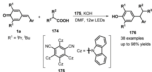
Scheme 36 Photocatalytic decarboxylation of carboxylic acids.
