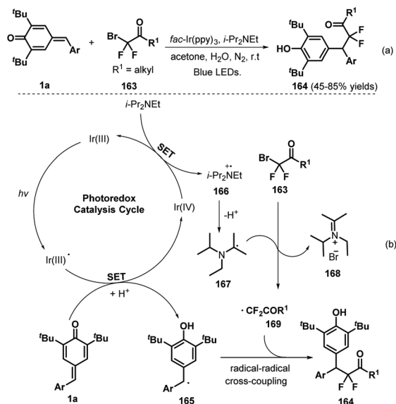
Scheme 33 Photocatalytic 1,6-hydrodifluoroacetylation of p -QMs.
