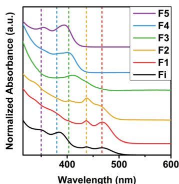
Fig. 4 Absorption spectra for the fraction obtained by size selective precipitation from the reaction mixture at 350 °C and 4.5 s. The table shows the absorption maxima of the CdSe species, their diameters and the calculated aggregation numbers. Fi is the initial sample and F1, ..., F5 the consecutive fractions obtained.
