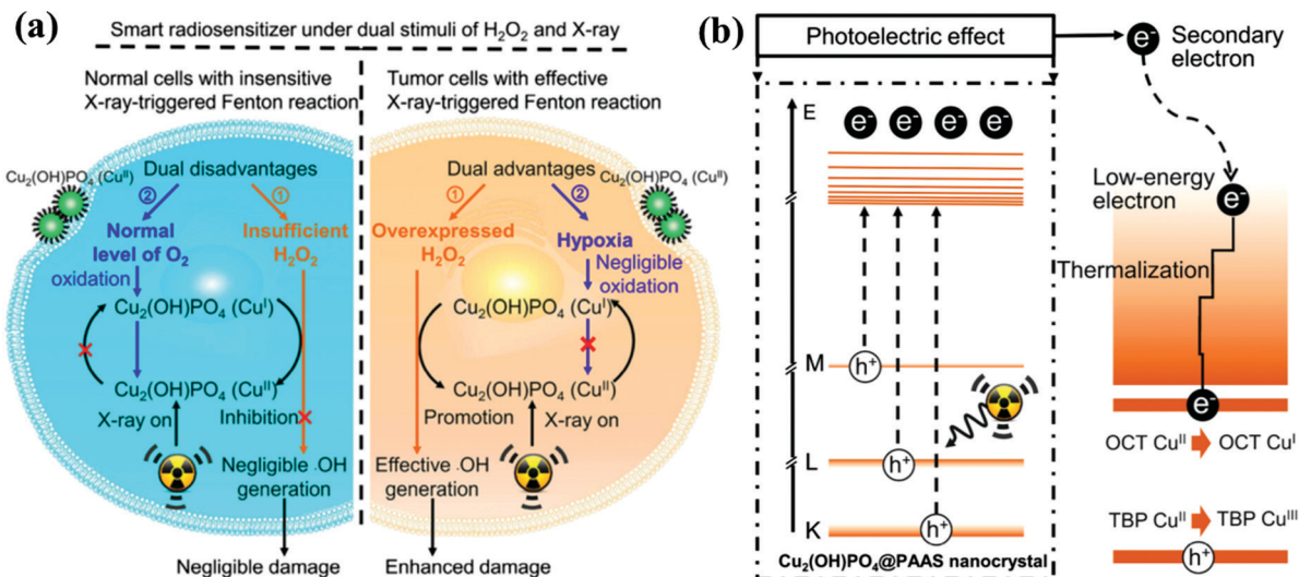
Fig. 3 (a) Schematic illustration of the as-constructed \text{Cu}_2(\text{OH})\text{PO}_4@PAAS nanocrystals for achieving an X-ray-triggered Fenton-like reaction just within the tumor microenvironment rather than the normal cells/tissue. (b) The scheme of the underlying mechanism for the generation of \text{Cu}^{\text{I}} sites in \text{Cu}_2(\text{OH})\text{PO}_4@PAAS nanocrystals by exogenous X-ray irradiation. 75 Copyright 2019, American Chemical Society.
