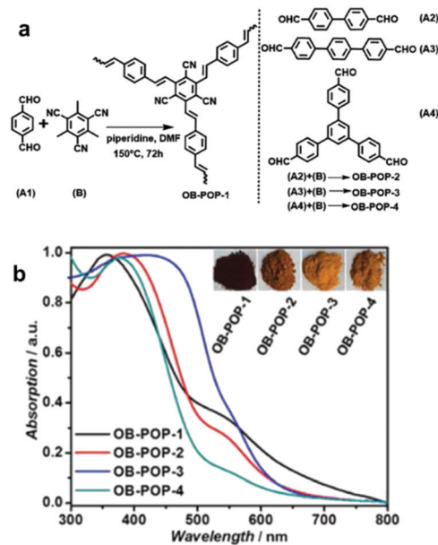
Fig. 2 Enhanced light absorbance using longer phenylene linkers in CPPs. (a) Synthetic process of olefin-bridged porous organic polymers (OB-POPs) and (b) their UV/vis diffuse reflectance spectra with photographs of the resulting polymers (inset). Reproduced with permission. 27 Copyright 2017 Wiley-VCH.
