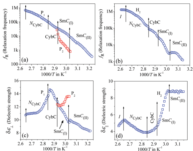
Fig. 5 Temperature dependence of the relaxation frequency ( f_R ) and dielectric strength ( \delta\epsilon ) for compound 1/10: (a and c) in planar and (b and d) homeotropic configurations, respectively. Vertical arrows define the corresponding phase-transition temperatures.
