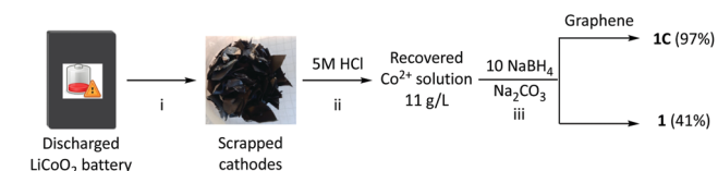
Scheme 2 Preparation sequence for 1 and 1C . (i) Manual dismantling and separation of cathode materials. (ii) Dissolution in 5 M \text{HCl} at 80 ^\circ\text{C} for 1 h. (iii) neutralisation and treatment with 10 eq. of \text{NaBH}_4 in ethanol, in the presence or absence of graphene.
