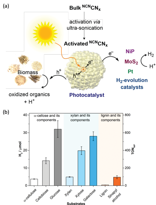
Fig. 6 (a) Schematic photo-reforming of lignocellulose using NCN CN x and proton reduction co-catalysts. (b) Photocatalytic H 2 production from purified lignocellulose components catalyzed by activated NCN CN x and NiP under AM1.5G light irradiation for one day at 25 °C. Reprinted from ref. 48 with permission of American Chemical Society, copyright 2018.
