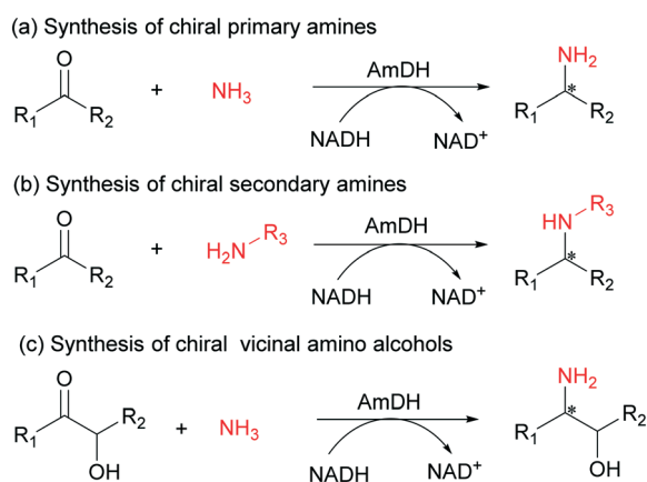
Scheme 1 Synthesis of chiral primary and secondary amines and chiral vicinal amino alcohols by AmDH-catalyzed asymmetric reductive amination of ketones and hydroxy ketones with ammonia or organic amines. AmDH, amine dehydrogenase.
