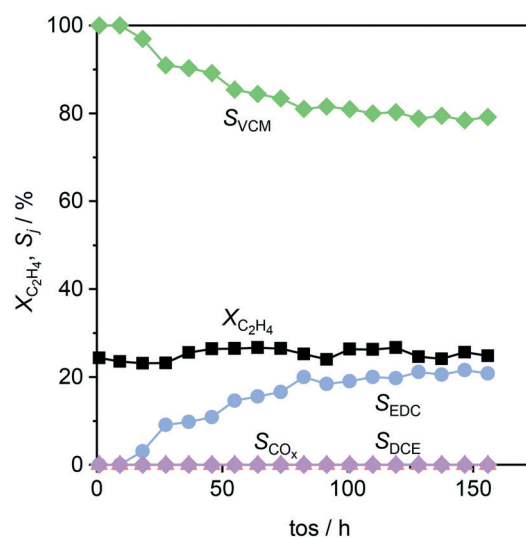
Fig. 10 Conversion and selectivity as a function of time-on-stream in ethene oxychlorination over a \text{CeO}_2/\text{ZrO}_2 - \text{Ca-I/Al}_2\text{O}_3 system as depicted in the fourth panel of Fig. 9. Conditions are detailed in Table 2.
