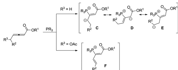
Scheme 1 The reactivity of allenates in the presence of organophosphines.
