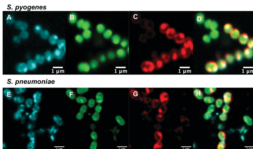
Fig. 3 Confocal microscopic images of (A–D) live resistant S. pyogenes (ATCC BAA-1412) and (E and F) resistant S. pneumoniae (ATCC 700676) labelled with (A and E) roxi-C 4 -Tz-DMACA 10 (10 µM); (B and F) Syto-9 (green nucleic acid dye, 5 µM); (C and G) FM4-64FX (red membrane dye, 5 µg mL -1 ); and (D and H) overlaid.
