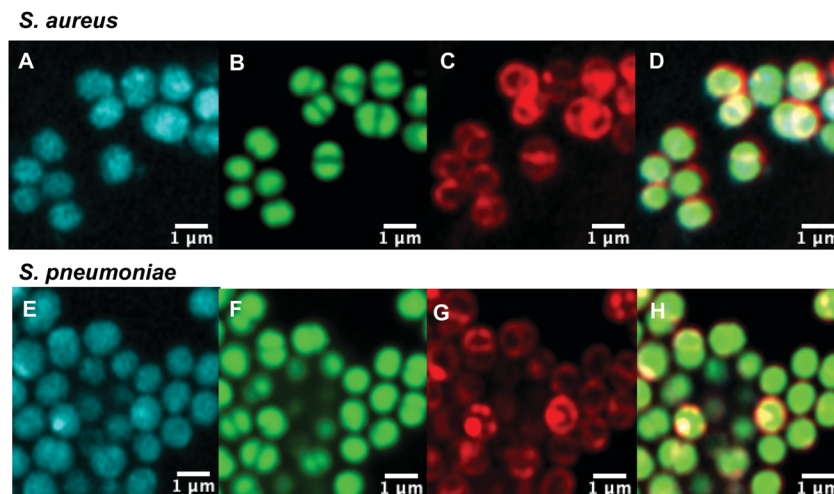
Fig. 2 Confocal microscopic images of (A–D) live susceptible S. aureus (ATCC 25923) and (E–H) susceptible S. pneumoniae (ATCC 33400) labelled with (A and E) roxi-C 4 -Tz-DMACA 10 (10 µM); (B and F) Syto-9 (green nucleic acid dye, 5 µM); (C and G) FM4-64FX (red membrane dye, 5 µg mL -1 ); and (D and H) overlaid.
