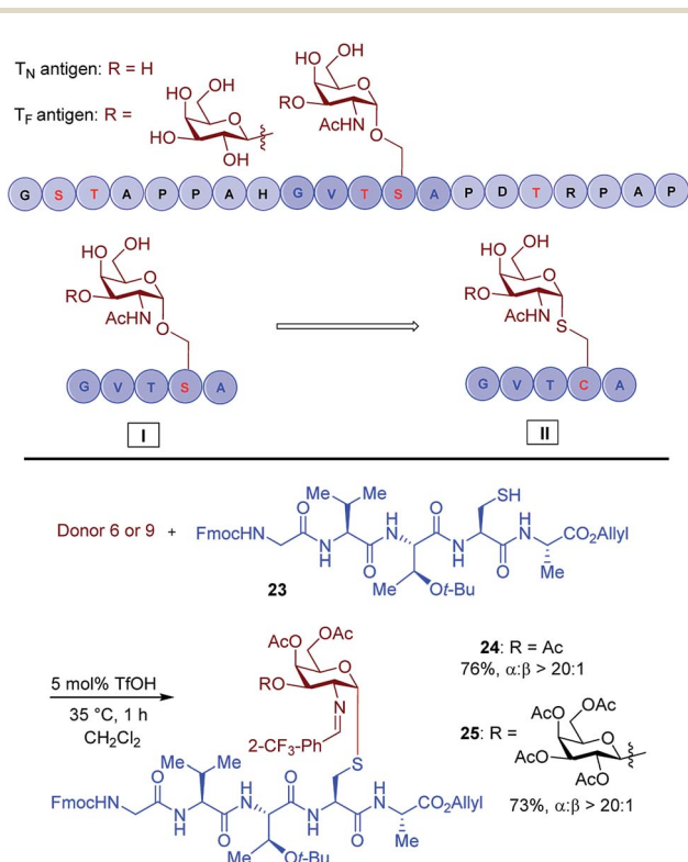
Scheme 3 Substrate synthesis of S -linked T N and T F glycopeptide fragments.
