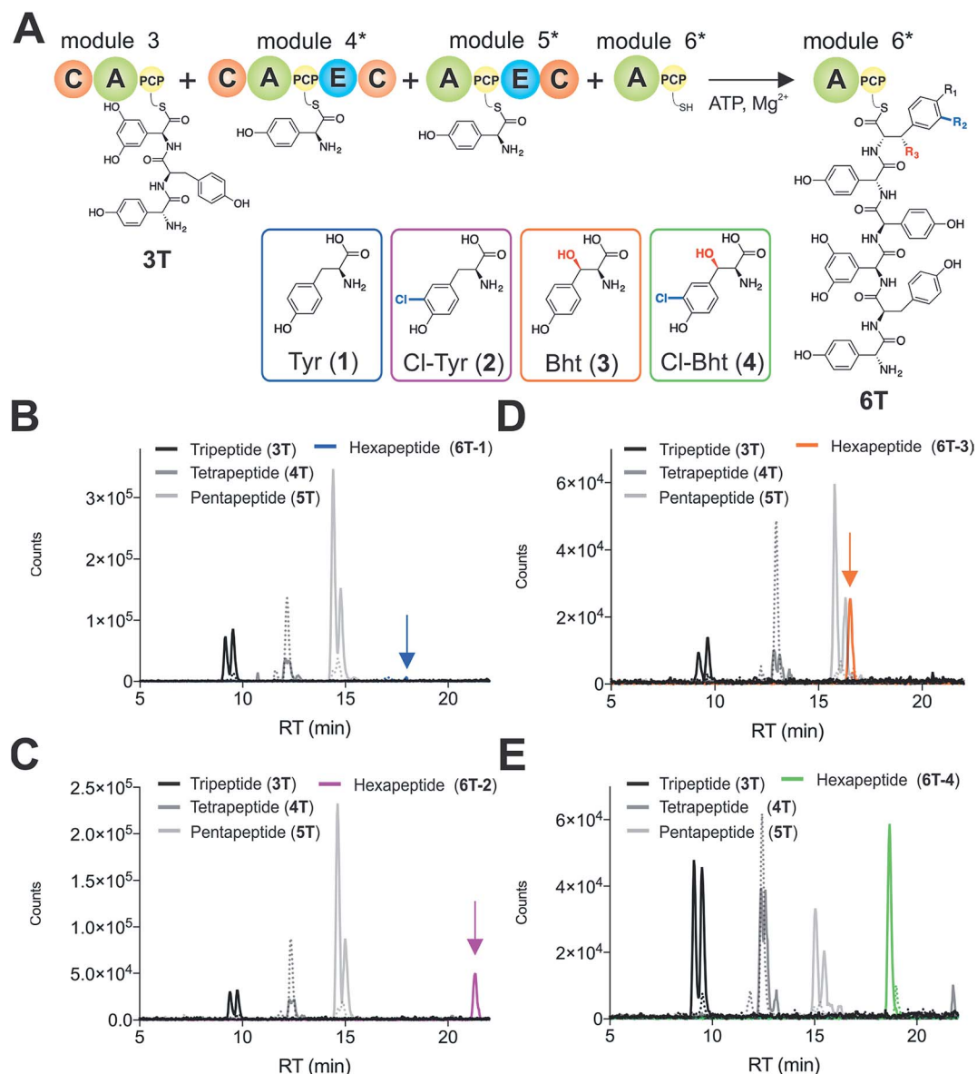
Fig. 5 Reconstitution of tripeptide extension using the separated modules (A-PCP-E-C architecture) from teicoplanin biosynthesis M3–M6 (Tcpl0/Tcpl1) using different substrates for module 6 (A). Peptide biosynthesis reconstituted using ATP, tripeptide (3T)-loaded M3, 4-Hpg, plus tyrosine (1) (B), Cl-Tyr (2) (C), Bht (3) (D) and Cl-Bht (4) (E) as M6 substrates, and determined by LCMS analysis (ESI, positive mode) with solid lines indicating methylamide peptides (PCP-bound) and dashed lines indicating hydrolysed peptides (tripeptide 3T: black line; tetrapeptide 4T: dark grey line; pentapeptide 5T: light grey line; hexapeptides 6T: blue line (Tyr, 6T-1), magenta line (Cl-Tyr, 6T-2), orange line (Bht, 6T-3) or green line (Cl-Bht, 6T-4)). A – adenylation domain, C – condensation domain, PCP – peptidyl carrier protein domain, E – epimerisation domain, Tyr – tyrosine (1), Cl-Tyr – 3-chlorotyrosine (2), Bht – \beta -hydroxytyrosine (3), Cl-Bht – 3-chloro- \beta -hydroxytyrosine (4).
