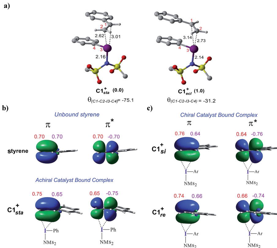
Fig. 5 (a) Optimized geometries of C1_{sta}^+ and C1_{eci}^+ . (b) Important natural bond orbitals (NBOs) corresponding to the \pi and \pi^* of (b) a free styrene as well as those in the iodine achiral catalyst–substrate complex C1_{sta}^+ , and (c) in the chiral catalyst–substrate complexes. Orbital coefficients on C_1 (in purple) and C_2 (in red) carbon atoms are given for each NBO.
