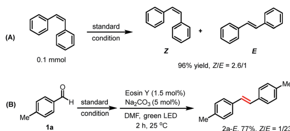
Scheme 4 Isomerization studies.
