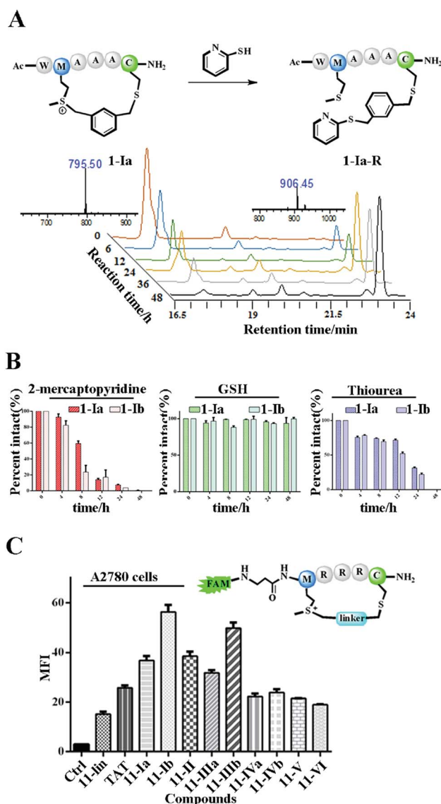
Fig. 2 The biochemical properties of the constrained peptides. (A) Dealkylation of model peptide 1-Ia (1 mM) in the presence of PyS (10 mM) in PBS (pH = 7.4) at 37 °C for 48 hours. HPLC traces of the time-dependent conversion between peptide 1-Ia and its conjugated product 1-Ia-R. (B) The kinetics of peptide dealkylation reactions with different reductants under the same reaction conditions as indicated in (A). (C) Cellular uptake of the cyclic and linear peptides in A2780 cells treated with 10 \mu\text{M} FAM-labeled peptides for 4 hours. All cells were incubated with 0.05% trypan blue for 3 minutes before further analysis.
