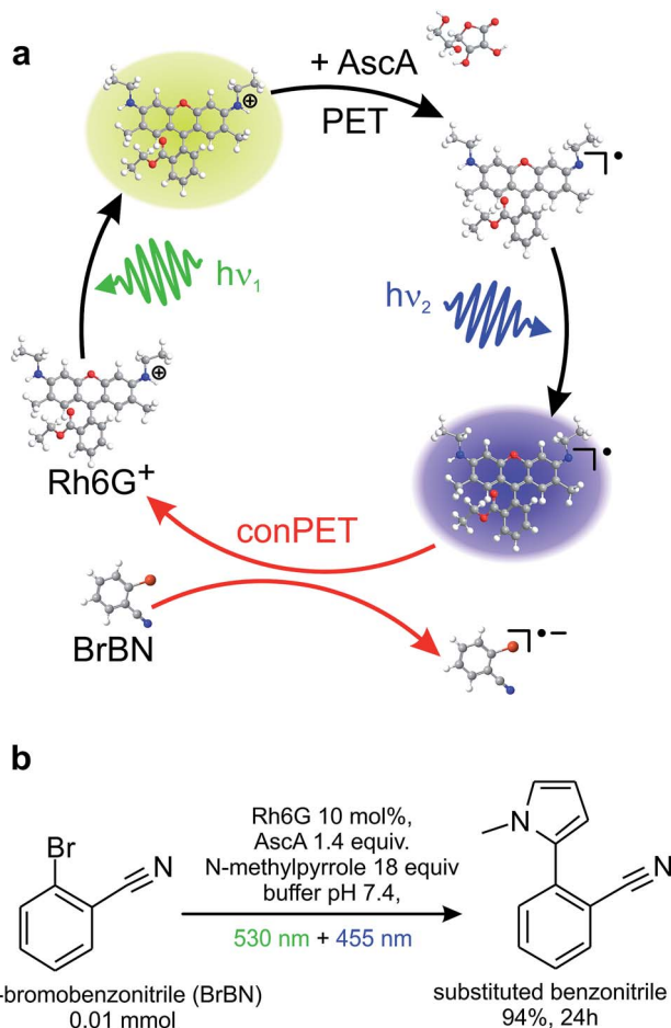
Fig. 1 A model dye-based photocatalytic reaction enabling addition of photon energy by consecutive photoelectron transfer (conPET). (a) A cationic rhodamine 6G (Rh6G) dye molecule in phosphate-buffered saline (PBS) is excited by a photon of energy h\nu_1 and is subsequently reduced by ascorbic acid (AscA) to form a radical. A second photon h\nu_2 excites the radical, leading to PET to the halogenated substrate 2-bromobenzonitrile (BrBN). Note that since in the single-molecule experiments it is the dye and not the product yield which is monitored, a trapping agent is not needed for this reaction. (b) Synthetic-scale C–H aromatic substitution of 2-bromobenzonitrile with an N -methylpyrrole trapping agent in an aqueous mixture of dye, substrate, reducing and trapping agent under two-colour LED illumination in the green ( h\nu_1 ) and blue ( h\nu_2 ). The conversion yield after 24 hours as determined by gas chromatography is 94%. Note that synthetic-scale reactions are usually carried out with LEDs rather than lasers. Lasers are necessary to focus light tightly in single-molecule experiments. Since the absorption spectrum of the radical state is broad, the reaction works for both blue wavelengths ( h\nu_2 ) of 405 nm (laser) and 455 nm (LED).
