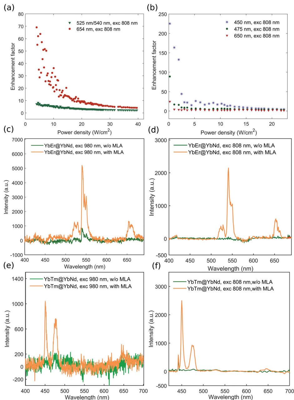
Fig. 3 Excitation intensity dependent enhancement factors induced by the addition of MLA of different emission bands of (a) \text{NaYF}_4:20\%\text{Yb}^{3+}, 2\%\text{Er}^{3+}@20\%\text{Yb}^{3+}, 30\%\text{Nd}^{3+} and (b) \text{NaYF}_4:20\%\text{Yb}^{3+}, 0.5\%\text{Tm}^{3+}@20\%\text{Yb}^{3+}, 30\%\text{Nd}^{3+} nanoparticles under 808 nm CW excitation. UCL spectra of \text{NaYF}_4:20\%\text{Yb}^{3+}, 2\%\text{Er}^{3+}@20\%\text{Yb}^{3+}, 30\%\text{Nd}^{3+} nanoparticles under (c) 980 nm and (d) 808 nm CW excitation with and without MLA light modulation (average excitation intensity: 0.1 \text{ W cm}^{-2} ). UCL spectra of \text{NaYF}_4:20\%\text{Yb}^{3+}, 0.5\%\text{Tm}^{3+}@20\%\text{Yb}^{3+}, 30\%\text{Nd}^{3+} nanoparticles under (e) 980 nm and (f) 808 nm CW excitation with and without MLA light modulation (average excitation intensity: 0.1 \text{ W cm}^{-2} ).
