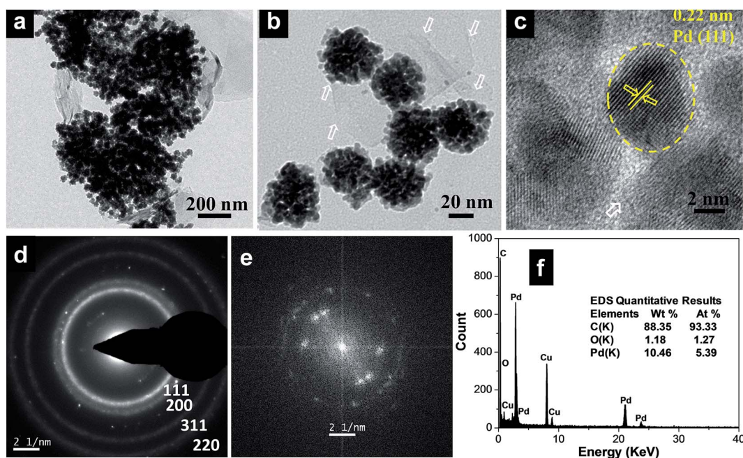
Fig. 1 (a and b) Transmission electron micrographs of the \text{Pd}_{100}/\text{GCN} nanohybrid at two different magnifications, (c) HRTEM image of palladium nanoparticles, (d) SAED pattern and (e) FFT and (f) EDS spectrum of the \text{Pd}_{100}/\text{GCN} nanohybrid. The white arrows represent the thin sheets of graphitic carbon.
