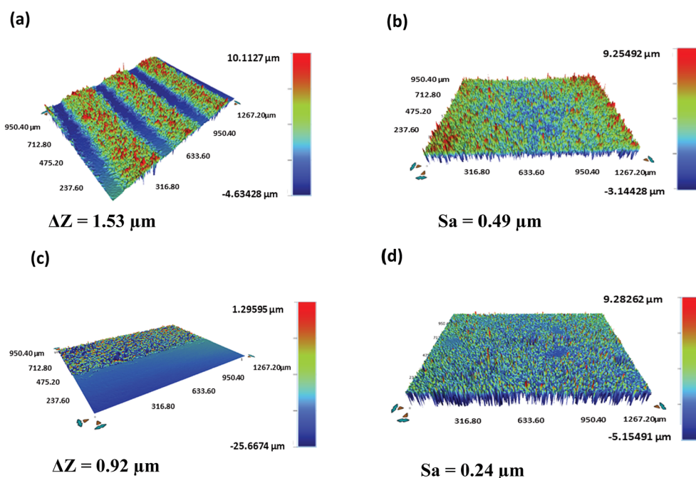
Fig. 6 3D output of the vertical scanning interferometry showing the (a) thickness and (b) roughness of silver electrodes and the (c) thickness and (d) roughness of the FMWCNT/HEC sensing layer.
