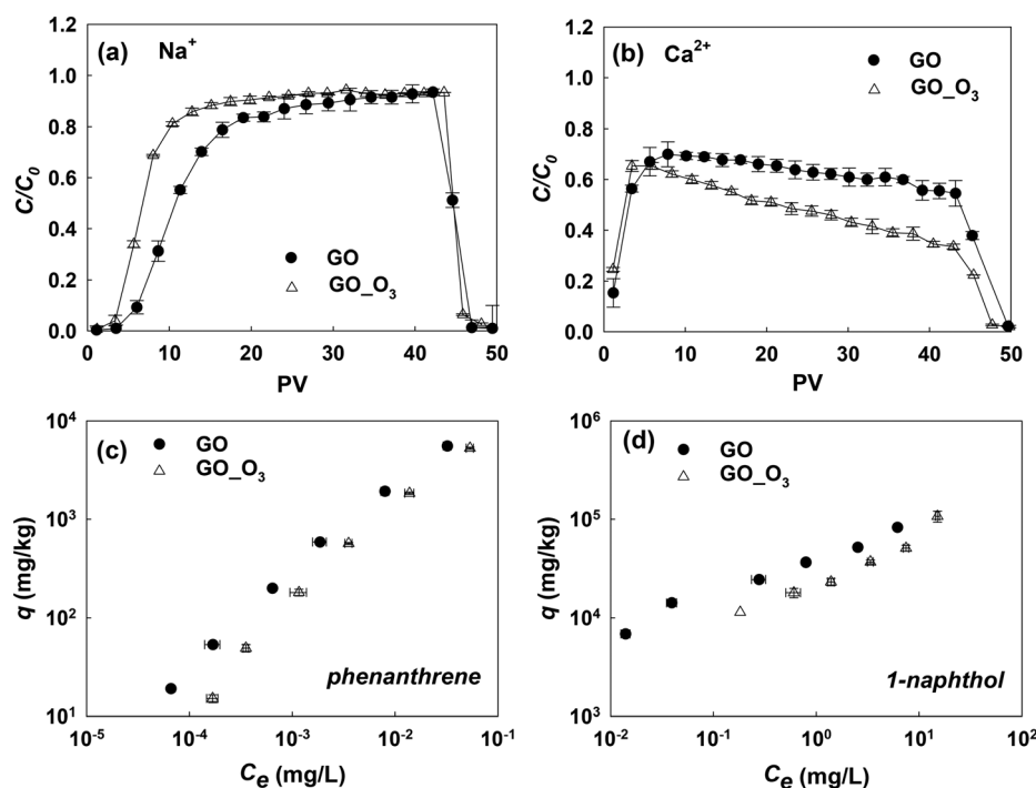
Fig. 6 Transport of GO and GO 03 in saturated quartz sand at (a) 35 mM NaCl (pH 6.0) and (b) 0.3 mM CaCl 2 (pH 6.0). C = concentration of GO in the effluent; C_0 = concentration of GO in the influent; C/C_0 , the ratio of the effluent concentration to the influent concentration. The data of breakthrough curves between 5 and 25 PV in the presence of Na + and after 10 PV in the presence of Ca 2+ were statistically significant by statistical analysis ( t -test, P < 0.05 ) performed with SPSS 22.0; adsorption isotherms of (c) phenanthrene and (d) 1-naphthol adsorbed onto GO and GO 03 . q (mg kg -1 ) and C_e (mg L -1 ) are equilibrium concentrations of contaminants on GO and in aqueous solution, respectively.
