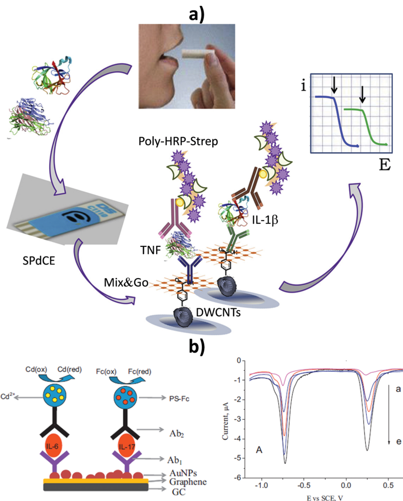
Fig. 16 Multiplexed electrochemical sandwich immunoplateforms using (a) multielectrode arrays or (b) barcode configurations. Simultaneous amperometric determination of TNF and IL-1 \beta at a SPdCE modified with 4-carboxyphenyl-functionalized double-walled carbon nanotubes (HOOC-Phe-DWCNTs) and polymeric coating Mix&Go to immobilize the capture antibodies in an oriented manner (a). Schematic illustration of the bioplateform developed for the simultaneous SWV determination of IL-6 and IL-7 using polystyrene spheres (PS) containing Cd 2+ or ferrocene (Fc) as tags (b, left). SWV traces recorded for simultaneous determination of increasing concentrations of IL-6 and IL-7 standards (b, right; from (a) to (e): 5, 50, 100, 500, 1000 \mu\text{g mL}^{-1} ). Reproduced and adapted from (a) ref. 19 and (b) ref. 184 with permission.
