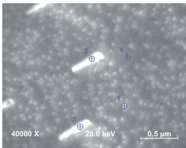
Fig. 5 SEM micrograph of the LSC64 pellet annealed at 800 °C in stagnant air for 2 h. Point 1 represents small size precipitates, and Points 2 and 3 represent large size precipitates. Point 4 represents the precipitate-free zone at the surface.
