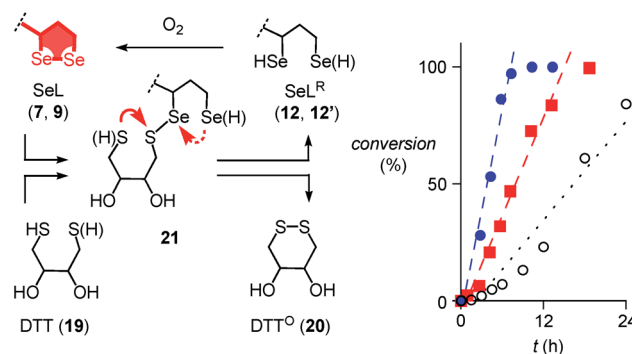
Fig. 4 Oxidation of 500 \mu\text{M} 19 to 20 as a function of time in the absence (○) and the presence of 500 \mu\text{M} 9 (■) and 22 (●) in \text{D}_2\text{O} , pD = 8.0 , with linear fits to determine the t_{50} . Structures are shown in neutral form, acidic protons are indicated in parenthesis. Competing ring closures in reactive intermediate 21 are indicated with solid (preferred) and dashed red arrows.
