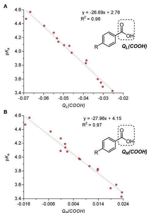
Fig. 7 (A) Correlation of benzoic acid pK_a with benzoic acid group L wdin partial charge Q_L(COOH) . (B) Correlation of benzoic acid pK_a with benzoic acid group natural population analysis (NPA) partial charge Q_N(COOH) .
