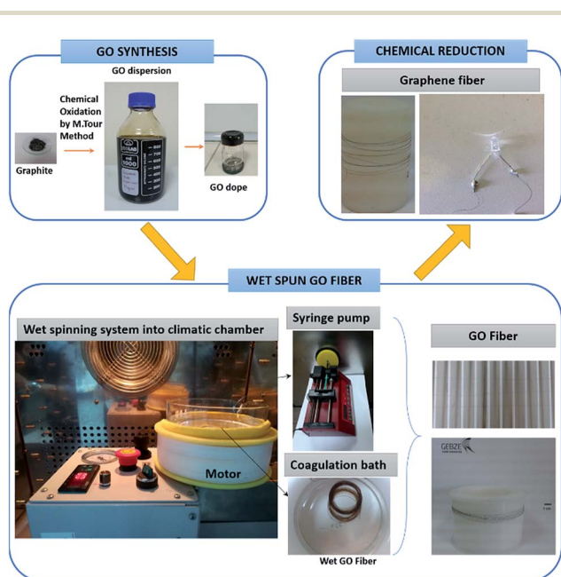
Fig. 1 Wet-spinning system to obtain GOFs and GF filament from graphite.
