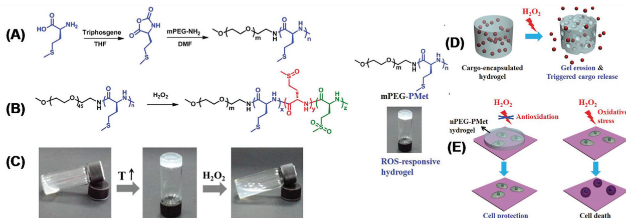
Fig. 7 (A) The synthetic route of poly(ethylene glycol)- b -poly(L-methionine) (mPEG-PMet). (B) Oxidation of the mPEG-PMet diblock copolymer by treating with \text{H}_2\text{O}_2 . (C) Photographs of the sol-gel transition with the increase of temperature and the gel disintegration by incubating with \text{H}_2\text{O}_2 . Schematic illustration of ROS-responsive mPEG-PMet hydrogels for oxidation-triggered cargo release (D) and cytoprotective effects (E) under oxidative stress. Reprinted with permission from ref. 61. Copyright (2016) WILEY-VCH.
