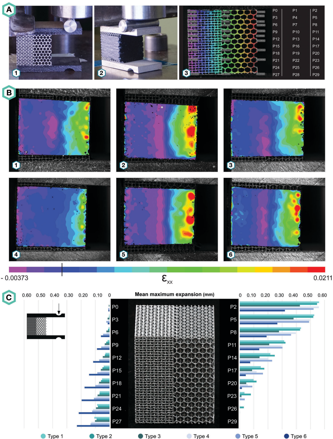
Fig. 3 Hybrid meta-biomaterials. (A) Test set-ups and image processing: (1) off-axis compression, (2) off-axis compression with an adherent layer used to improve visualization of strain distribution, (3) points plotted along the borders of a hybrid meta-biomaterial and the order in which they were numbered according to their position. (B) Horizontal strains in the tape surrounding hybrid meta-biomaterials types 1–6 at 2 mm displacement. (C) Mean maximum expansion during off-axis compression.
