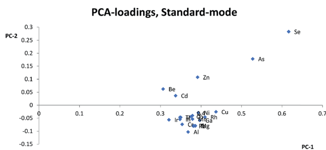
Fig. 5 Weighted PCA loadings according to explained variance including all matrixes in standard-mode, based on centered \ln(x) transformed data for 9 Be, 24 Mg, 27 Al, 49 Ti, 51 V, 53 Cr, 55 Mn, 59 Co, 61 Ni, 65 Cu, 67 Zn, 69 Ga, 75 As, 82 Se, 89 Y, 103 Rh, 111 Cd, 115 In, 193 Ir, 205 Tl, 208 Pb.
