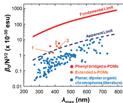
Fig. 2 Intrinsic \beta vs. \lambda_{\text{max}} for 1 , 2 and 3 vs. short (phenyl bridged) POMophores, 5 and planar, dipolar organic chromophores. 7 Compound 2 is the first POMophore to clearly breach Kuzyk's apparent limit for the performance of planar, dipolar organic chromophores.
