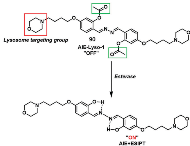
Scheme 79 An AIE + ESIPF probe 90 that allows for the monitoring of lysosomal esterase activity in MCF-7 cells. Measurement conditions: PBS buffer solution (pH = 7.4). Reproduced with permission from ( J. Mater. Chem. B , 2014, 2 , 3438–3442). Copyright (2014) the Royal Society of Chemistry.
