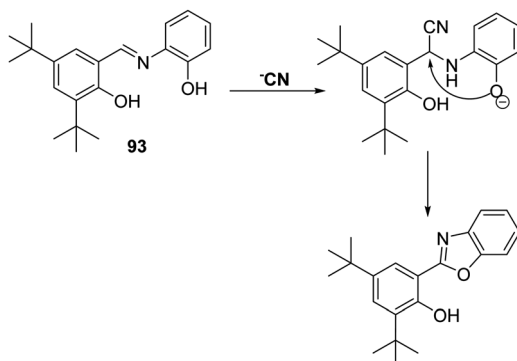
Scheme 82 Schiff-base fluorescent probe 93 . This system undergoes a cyanide anion-induced oxidative cyclisation to form an active ESIPF fluorophore, HBO. Measurement conditions: H 2 O containing CTAB.
