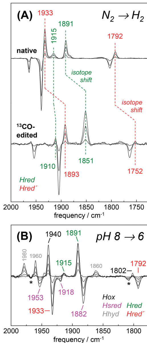
Fig. 6 Reduction of HYDA1 ^{\text{adt}} in the presence of \text{H}_2 . (A) IR difference spectra in the CO region collected during a change from 100% \text{N}_2 to 10% \text{H}_2 on native (top) and ^{13}\text{CO} -edited HYDA1 ^{\text{adt}} (bottom). Spectra show an increase of Hred (green) and Hred' (red) at the expense of Hox (black). Isotope editing of the \mu\text{CO} and dCO ligands leads to \sim 40 \text{cm}^{-1} frequency down-shifts in Hox , Hred , and Hred' . (B) Difference spectra for changing the pH from 8 to 6 in the presence of 10% \text{H}_2 (for absolute spectra see Fig. S10, ESI ^\dagger ). Here, Hred (green) and Hox (black) are populated at the expense of Hred' (red) and Hsred (magenta). Note the additional formation of Hhyd (grey) and decrease of the minor Hox-CO population (asterisks).
