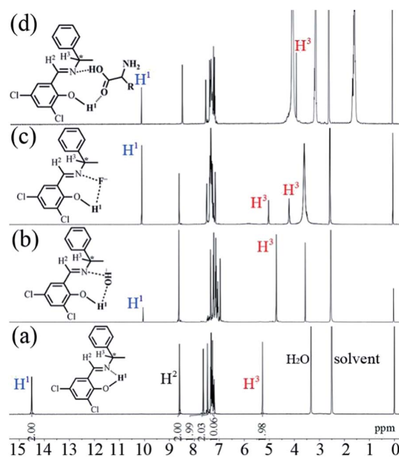
Fig. 11 1 H NMR spectra of 3,5-Cl-diPh (a), 3,5-Cl-diPh + 100 equivalent of OH - (b), 3,5-Cl-diPh + 100 equivalent of F - (c), and 3,5-Cl-(R,R)diPh + 100 equivalent of L-Arg (d) in DMSO-d 6 .
