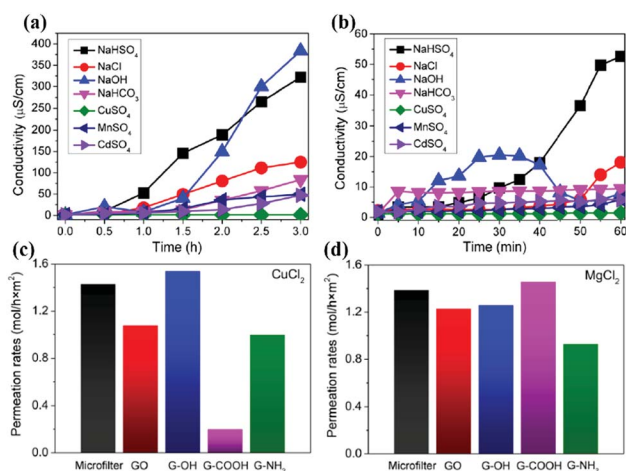
Fig. 6 (a) Penetration processes of different ionic compounds through graphene oxide membranes; 57 (b) initial stages of the penetration processes; 57 (c) Cu^{2+} and (d) Mg^{2+} permeation rates through different membranes. 58,59
