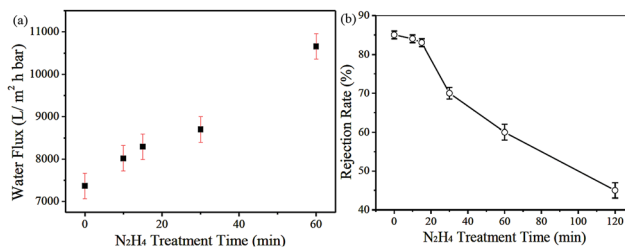
Fig. 23 (a) Water flux and (b) rejection rate of EB molecules of GO/CHNs membrane with \text{N}_2\text{H}_4 treatment for different durations. 85
