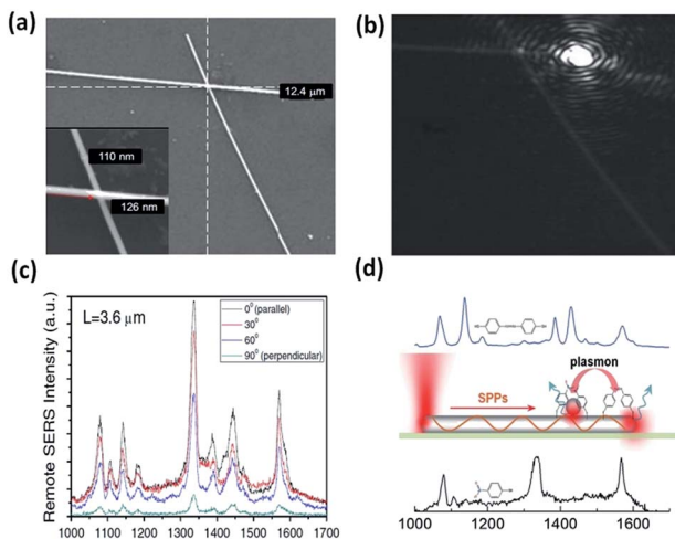
Fig. 14 (a) SEM image of intersecting Ag nanowires. (b) Dark field image of crossed Ag nanowires. The big white spot is incident light and the tiny spot is the emitting light. (c) The polarization-dependent remote surface catalytic reaction of 4-NBT. (d) Schematic illustration of 4-NBT converted to DMAB by propagating SPPs, where the surface plasmons exit at one terminal and the Raman signal is collected at the other terminal of an Ag nanowire. 77
