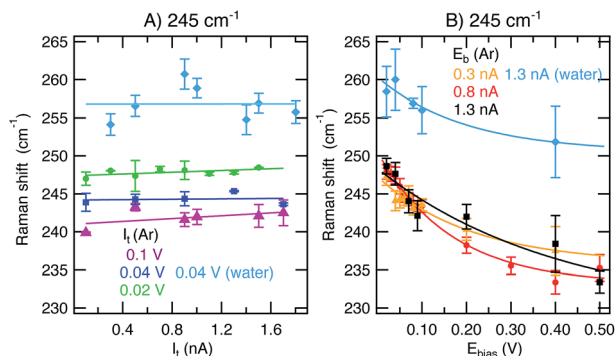
Fig. 4 Raman shift of the 245 cm -1 mode as a function of I_t ((A), at constant E_b values of 0.02 V, green circles; 0.04 V, dark blue squares; 0.1 V in Ar, purple triangles; and 0.04 V in water, light blue diamonds) or E_b ((B), at constant I_t values of 0.3 nA, orange triangles; 0.8 nA, red circles; 1.3 nA in Ar, black squares; and 1.3 nA in water, light blue diamonds). Averaged results from spectra taken in scans up and down are presented with the standard deviation as the error. Solid lines are included as a guide to the eye.
