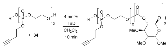
Fig. 32 Block copolymers of 34 showing stimuli sensitive phase behaviour (R = 4-MeBn).
