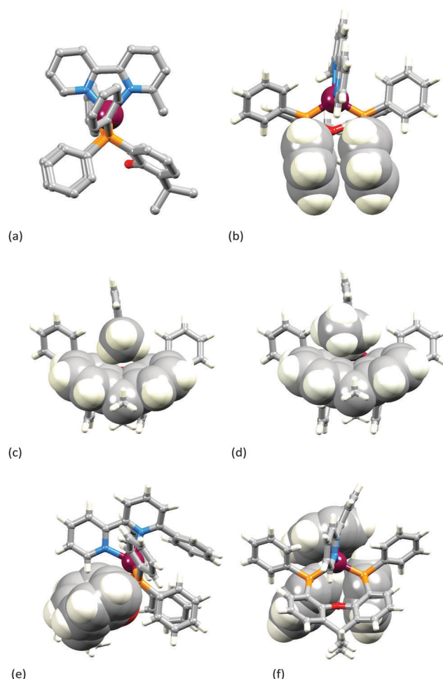
Fig. 3 (a–c) The structure of the [\text{Cu}(\text{xantphos})(\text{Me bpy})]^+ cation: (a) view along the P–P vector of the xantphos ligand (H atoms omitted for clarity); (b) face-to-face \pi -stacking of phenyl rings in the two different \text{PPh}_2 units; (c) accommodation of the methyl group of Me bpy in the xantphos 'bowl'. (d) A view of the [\text{Cu}(\text{xantphos})(\text{Et bpy})]^+ cation for comparison with the analogous view of [\text{Cu}(\text{xantphos})(\text{Me bpy})]^+ shown in (c). (e and f) The structure of the [\text{Cu}(\text{xantphos})(\text{Ph bpy})]^+ cation with space-filling representations emphasizing (e) the xanthene 'bowl' with the unsubstituted pyridine ring lying above it, and (f) the phenyl group of Ph bpy oriented over two Ph rings of the \text{PPh}_2 units.
