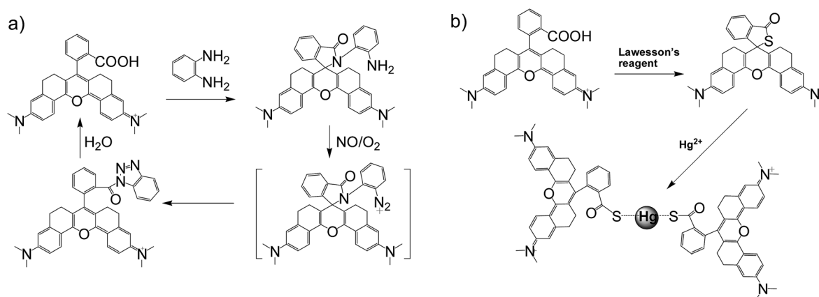
Scheme 2 (a) NO-induced ring opening of HN7-N2 . (b) \text{Hg}^{2+} -induced ring opening of HN7-S .
