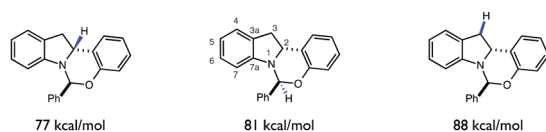
Fig. 10 Uncorrected bond energies for C–H bonds of 1 (UB3LYP/6-311+g(d,p)).
