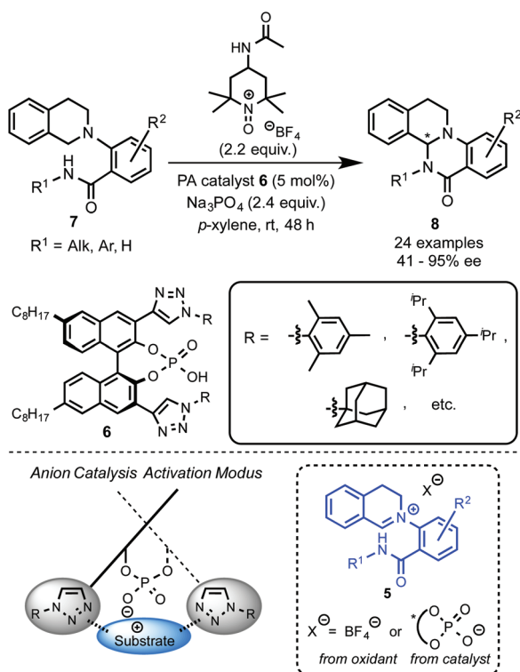
Scheme 5 Chiral phosphate catalysis in \text{C}(\text{sp}^3) -H functionalization.
