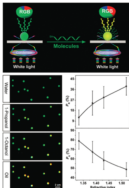
Fig. 3 (Top) Schematic illustration of the dark-field scattering signal interpreted into tricolor RGB values. (Bottom left) Scattering images of gold NPs immersed in solvents with different refractive indexes, showing the green dots for water gradually turned yellow. (Bottom right) Results of RGB analysis showing that as the refractive index of the surrounding solvent increases, the red component (PR) increases while the green component (PG) decreases. (Reprinted with permission from ref. 68.)
