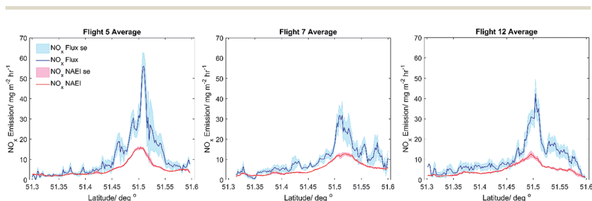
Fig. 5 Average for Flights 5, 7 and 12, measured NO x flux plotted in blue with standard error as the shaded blue area. Calculated and scaled NAEI estimates of NO x emission are plotted in red, with standard error as the shaded red area.
