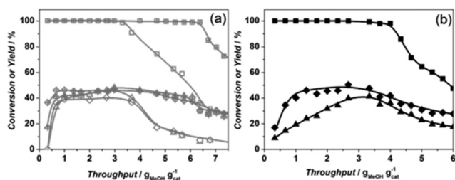
Fig. 8 Methanol conversion (■), ethylene (▲) and propylene (◆) yields of (a) Sigma1-315-S (□, △, ◇) and Sigma1-315-S-m (⊞, ⊠, ⊡); (b) ZSM-58 (■, ▲, ◆) ( \text{SiO}_2/\text{Al}_2\text{O}_3 = 110 , 0.6\text{--}1.8 \mu\text{m} ) at 450 \text{ }^\circ\text{C} and standard operation conditions.
