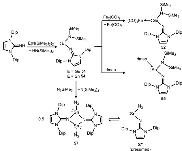
Scheme 12 Preparation of amino(imino)metallylenes 51 and 54 and the iron carbonyl 52 , as well as the dmap adduct 55 ( dmap = 4-dimethylamino-pyridine). Conversion of 54 to dimeric stannyliumylidene azide 57 .
