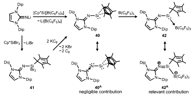
Scheme 9 Synthesis of \text{Cp}^* -substituted iminosilylene 40 and its borane adduct 42 , as well as the dibromide precursor 41 . Silylene–nitrene formulation 40 A and sila-2-aza-allene canonical structure 42 A .
